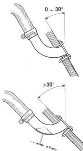
Installation to the stern side
